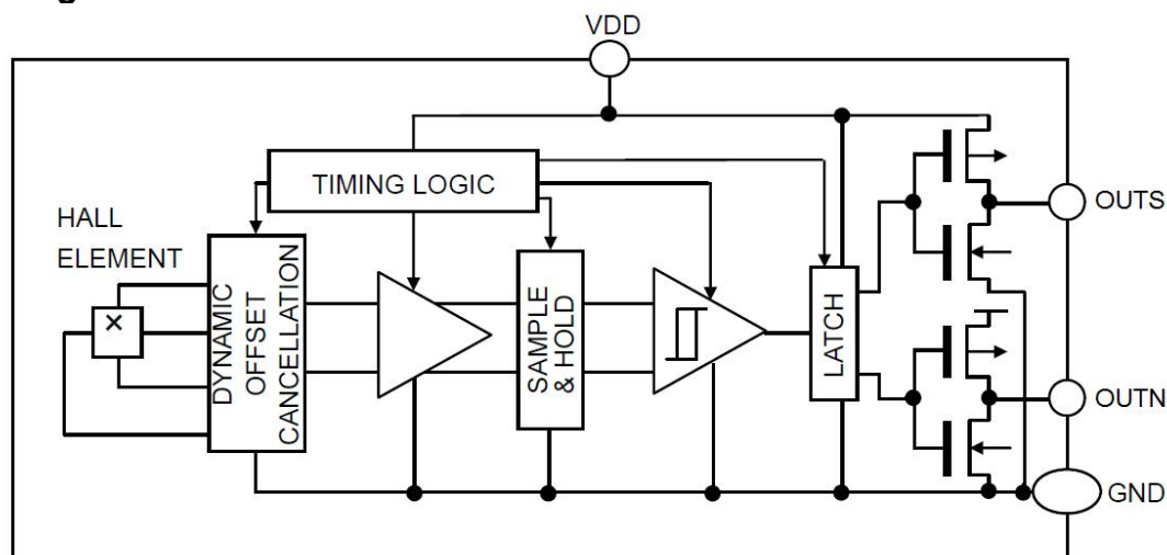
Figure 2, Block Diagram of AS1826
