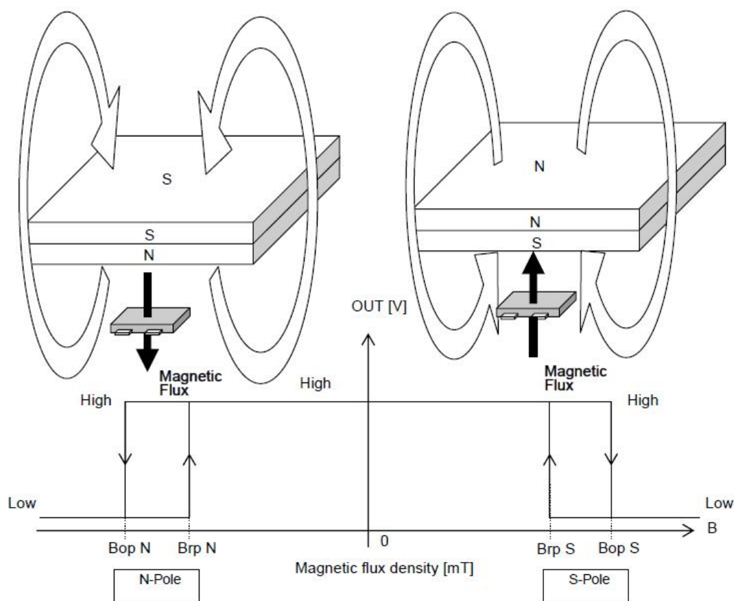
Figure 3, Magnetic Operation Characteristic of AS1826
