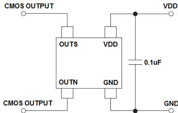
Figure 1, Typical Application Circuit of AS1826
